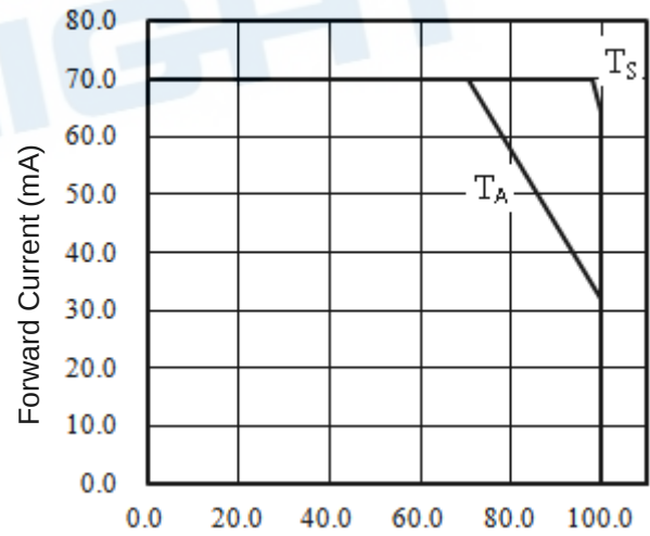
Max. Permissible Forwarded Current ( T_a=25^\circ\text{C} )
