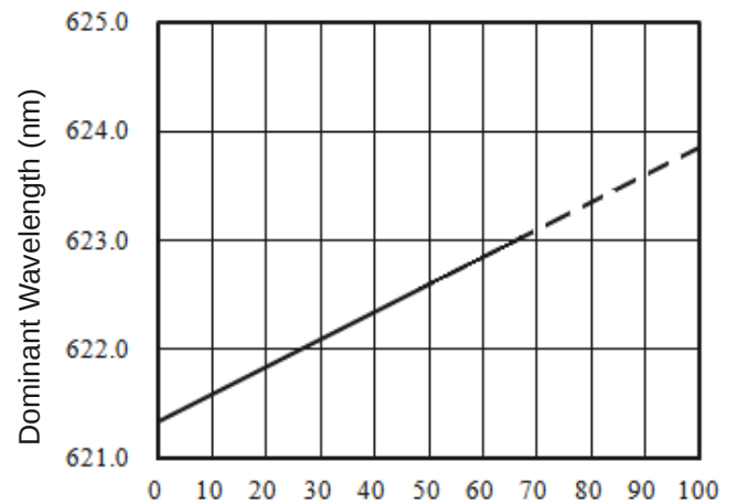
Dominant Wavelength vs. Forward Current ( T_a=25^\circ\text{C} )
