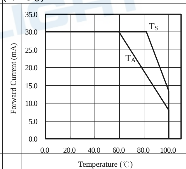
Max. Permissible Forwarded Current ( T_a=25^{\circ}\text{C} )
