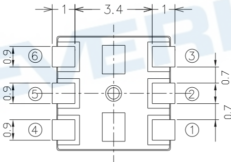
Bot. view
