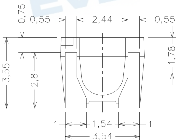
Bot. view
