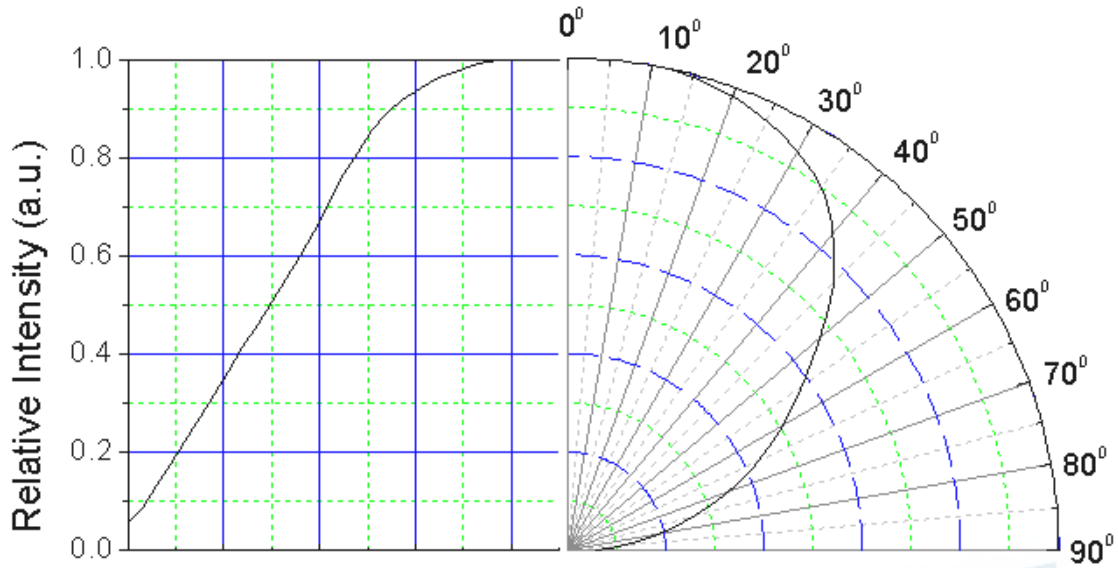
Shwo(F) series: Typical Diagram Characteristics of Radiation
