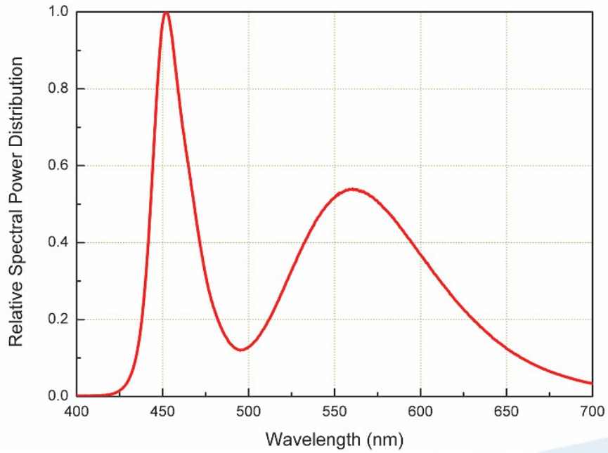
Cool-White @ Thermal Pad Temperature = 25°C
