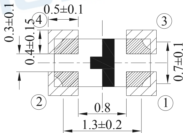
Recommend Soldering Pad
