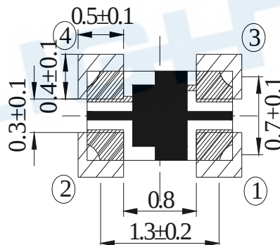
Recommend Soldering Pad
