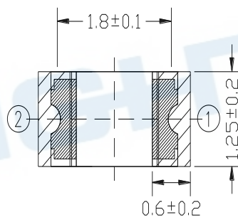
Recommend Soldering Pad
